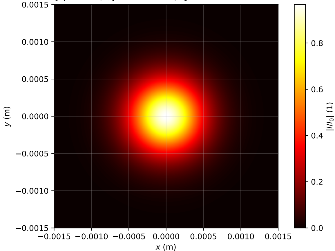
Intensity profile I(x, y, z = 1.115m)/I_0 , P_{in}=0.4P_{cr} , artificial time
